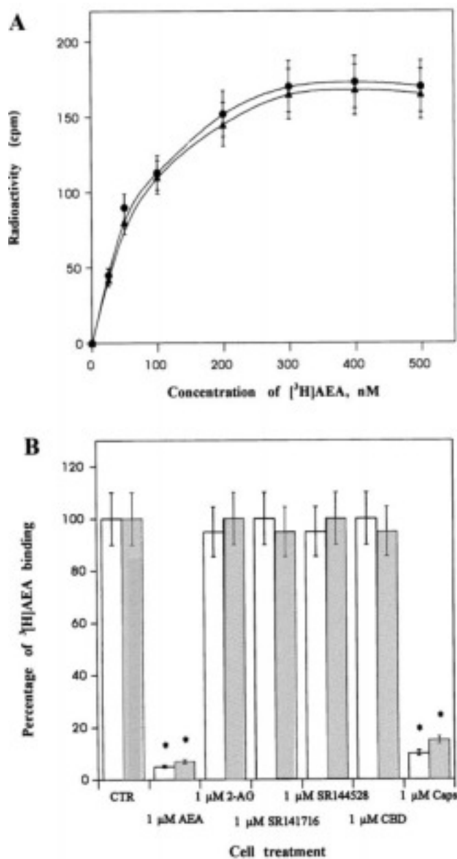
FIG. 3. Binding of AEA to CHP100 and U937 cells. A, represents the binding of [ 3 H]AEA to CHP100 (circles) or U937 (triangles) cells. B, the effect of (cold) AEA, 2-AG, SR141716, SR144528, CBD, or Caps (each used at 1 μM) on the binding of 200 nM [ 3 H]AEA to CHP100 (white bars) or U937 (gray bars) is shown, and values were expressed as percentage of the untreated controls (100% = 170 ± 20 (CHP100) or 160 ± 20 (U937) cpm, respectively). CTR, control. *, p < 0.01 compared with control cells.
