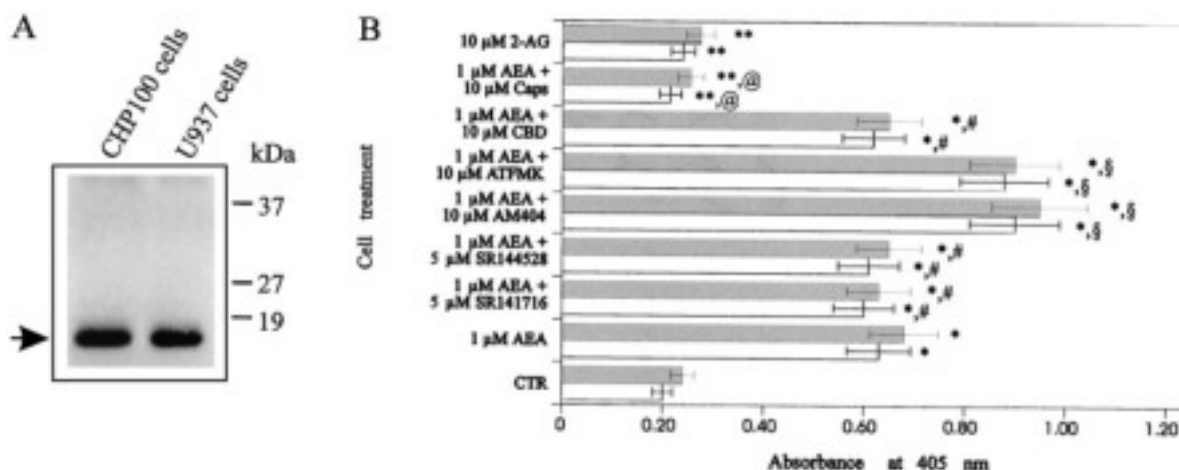
FIG. 4. Effect of AEA on cytochrome c release from CHP100 and U937 cells. A shows Western blot analysis of cytochrome c in cell homogenates (25 \mu\text{g}/\text{lane} ). The arrow indicates the expected molecular size for cytochrome c. Molecular mass markers are shown on the right-hand side. B shows the effect of 1 \mu\text{M} AEA, in the absence or in the presence of 5 \mu\text{M} SR141716, 5 \mu\text{M} SR144528, 10 \mu\text{M} AM404, 10 \mu\text{M} ATFMK, 10 \mu\text{M} CBD, or 10 \mu\text{M} Caps, on cytochrome c release from CHP100 (white bars) or U937 (gray bars) cells, as determined by ELISA at 405 nm (see "Experimental Procedures"). Treatment of either cell line with any of the compounds listed, in the absence of AEA, was ineffective under the same experimental conditions. CTR, control. *, p < 0.01 compared with control cells; **, p > 0.05 compared with control cells; #, p > 0.05 compared with AEA-treated cells; §, p < 0.05 compared with AEA-treated cells; @, p < 0.01 compared with AEA-treated cells.
